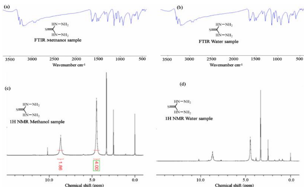
Fig. 1. FTIR and ^1\text{H} NMR for thiocarbohydrazide prepared through methanol and water synthetic pathways
