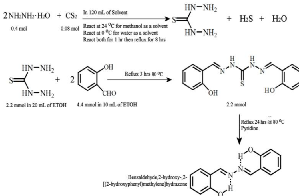
Fig. 6. Synthetic pathways of thiocarbohydrazide and benzaldehyde,2-hydroxy-,2-[(2-hydroxyphenyl) methylene]hydrazine compounds
