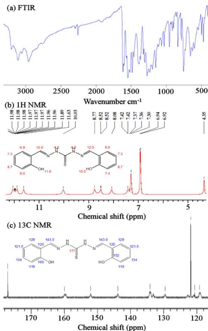
Fig. 3. FTIR (a), ^1\text{H} NMR (b) and ^{13}\text{C} NMR (c) for 1,5-bis (2-hydroxybenzaldehyde) dithiocarbohydrazone
