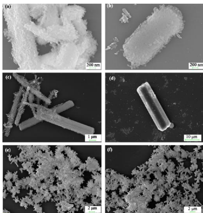
Fig. 2. Morphological differences between thiocarbohydrazide prepared in water (a, b), and in methanol (c, d) as reaction solvents. The monograms were taken after the two samples were powdered. Morphologies in (e and f) are for both samples after recrystallization in water
