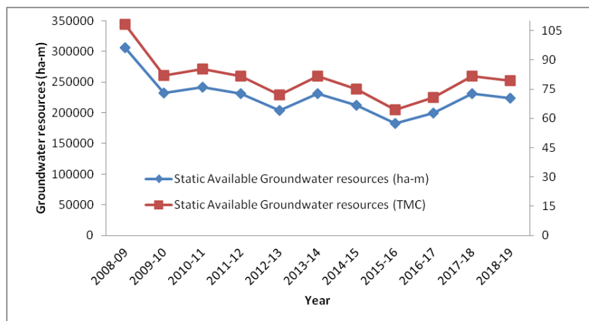
Fig. 4. Available groundwater volume of NSRC command area
