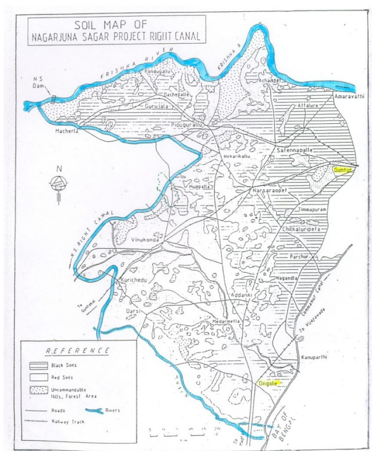
Fig. 2. Soils distributed over the NSRC Command Area
